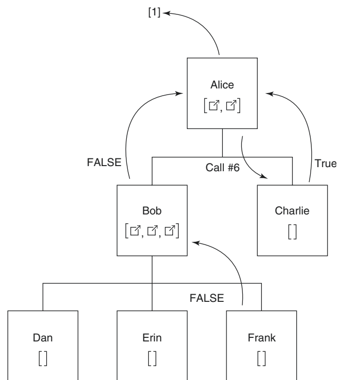
Fig. 2.7 Returning the result
