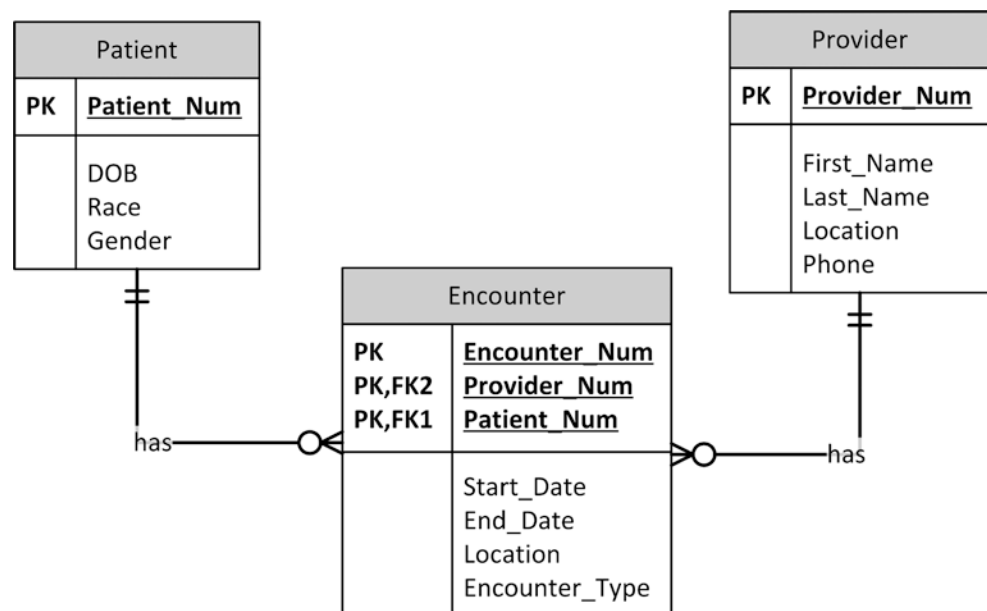
Fig. 10.1 Entity relationship diagram for a simple database schema
