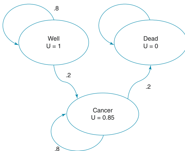
Fig. 6.9 A simple Markov model. The Markov model shows three health states, well , cancer , and dead . Arcs (arrows) between the health states represent the probability of transitioning from one health state to the next during a Markov cycle (for example, a year). Utility is accumulated for each cycle (see Table 6.4)
